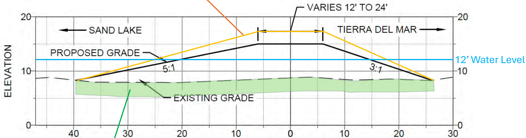
SETBACK DIKE TYPICAL SECTION
