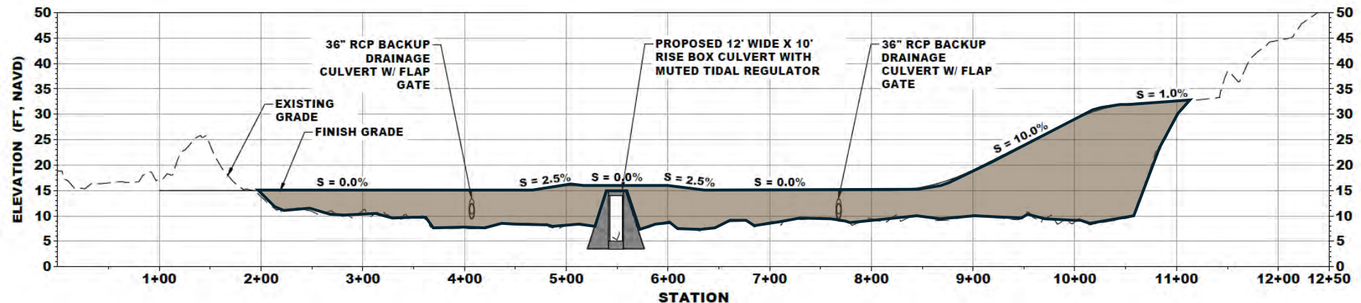
SETBACK DIKE PROFILE PROFILE HORIZONTAL SCALE: 1" = 50' VERTICAL SCALE: 1" = 10'
