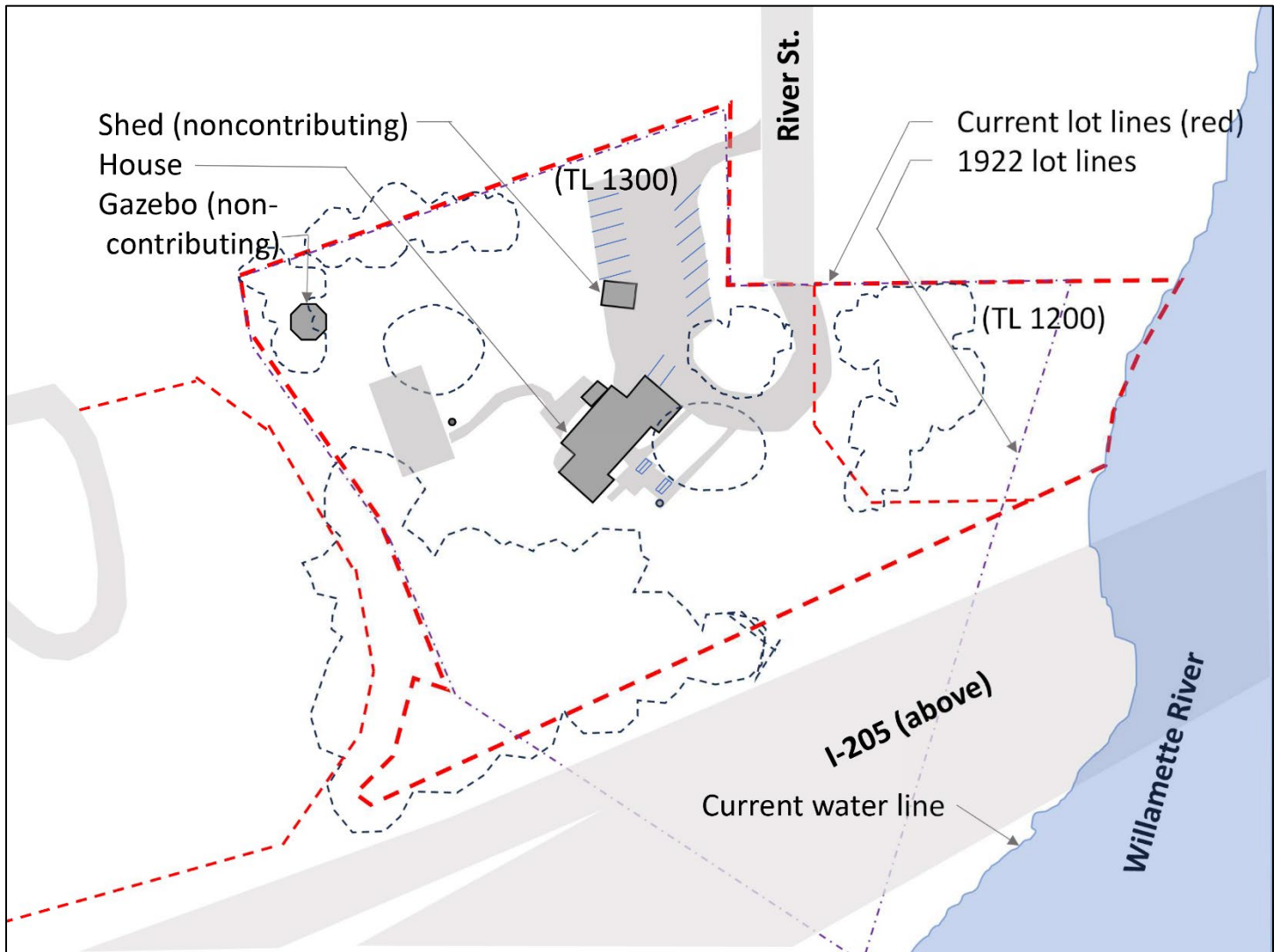
Figure 4: Site plan
