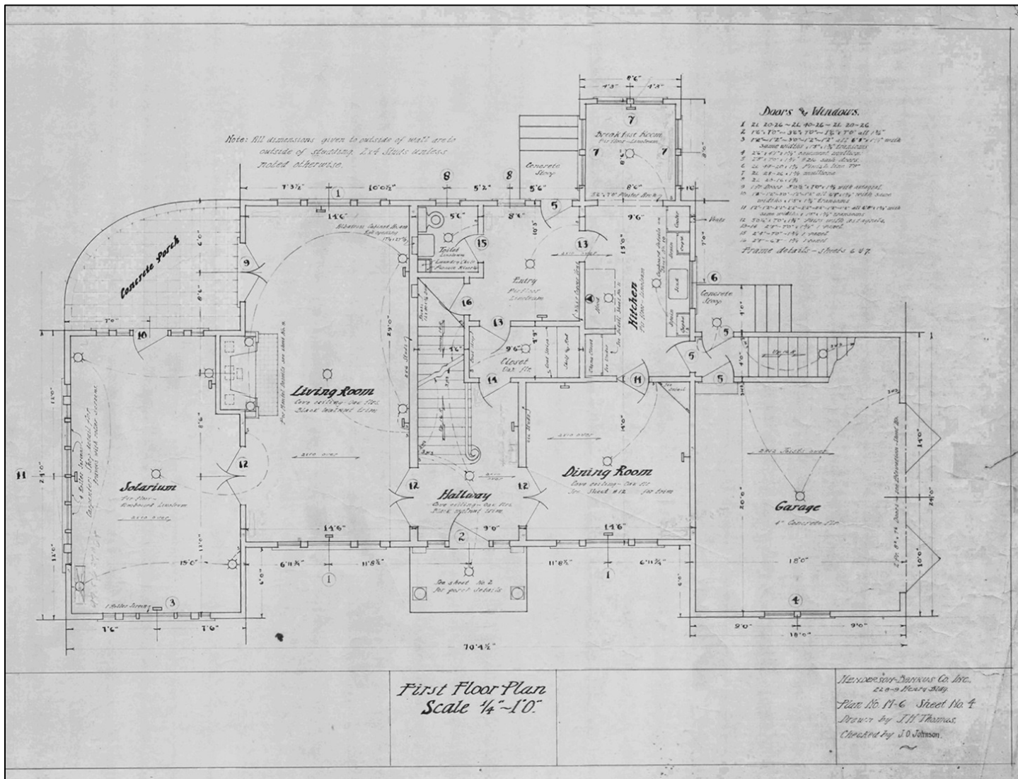
Figure 5: Main level plan drawing, c.1927, of Dr. and Mrs. E. H. McLean House by Henderson-Bankus Company, Inc. Plan is unchanged as of 2024 except for extension of breakfast room roof over back stoop.
