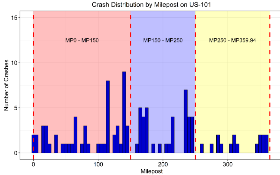
Figure 5.9: Crash distribution by milepost on US-101
