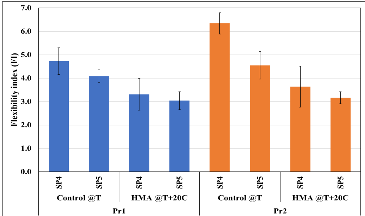
Figure 4.3. The impact of increased mixing and compaction temperatures on cracking resistance (length of the error bar is equal to one standard deviation).
