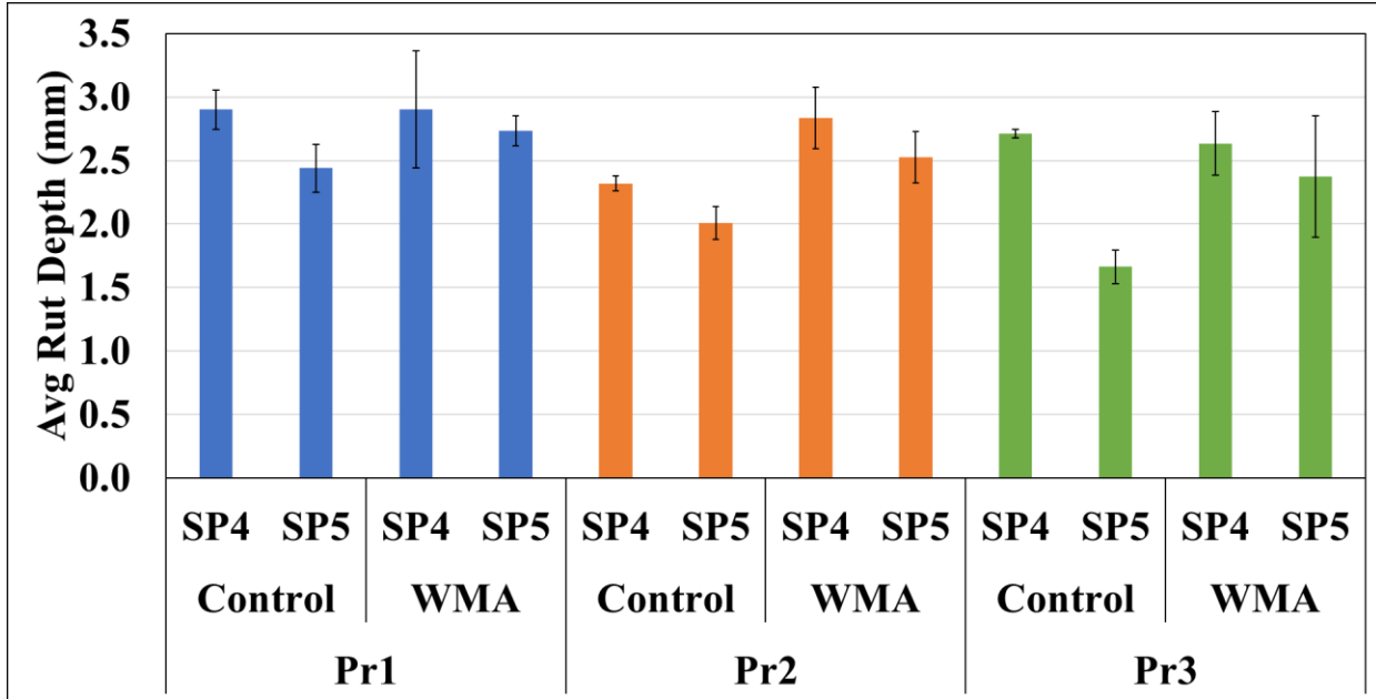
Figure 4.4. HWTT test results for the HMA (control) and WMA mixes prepared with two different design methods, SP4 and SP5 (length of the error bar is equal to one standard deviation).
