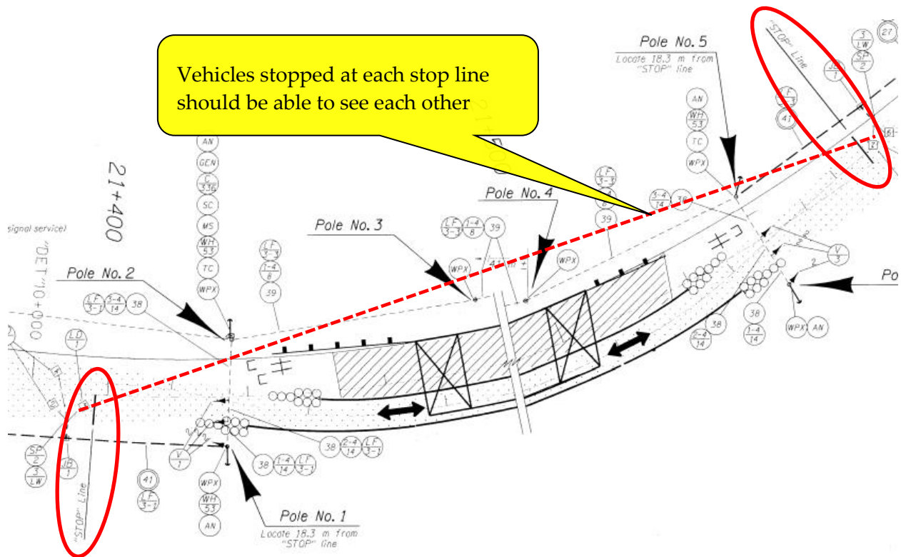
Figure 11-22 | Sight Distance from Stop Line to Stop Line
