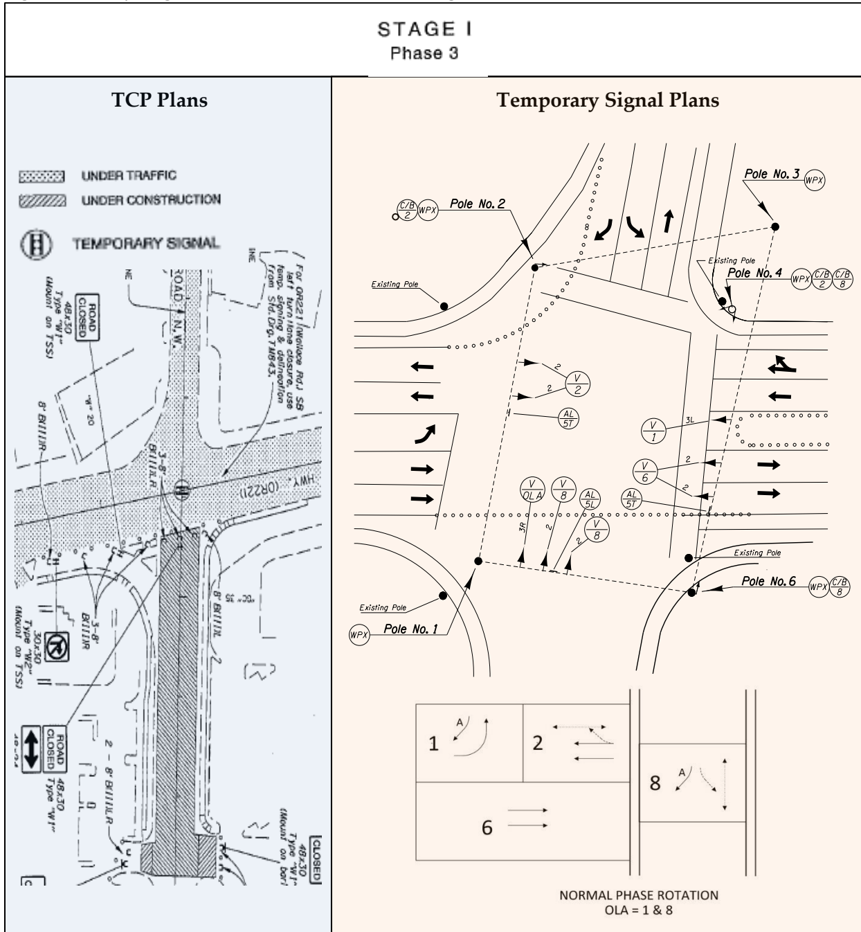
Figure 11-13 | Staged Construction Example – Stage I, Phase 3
