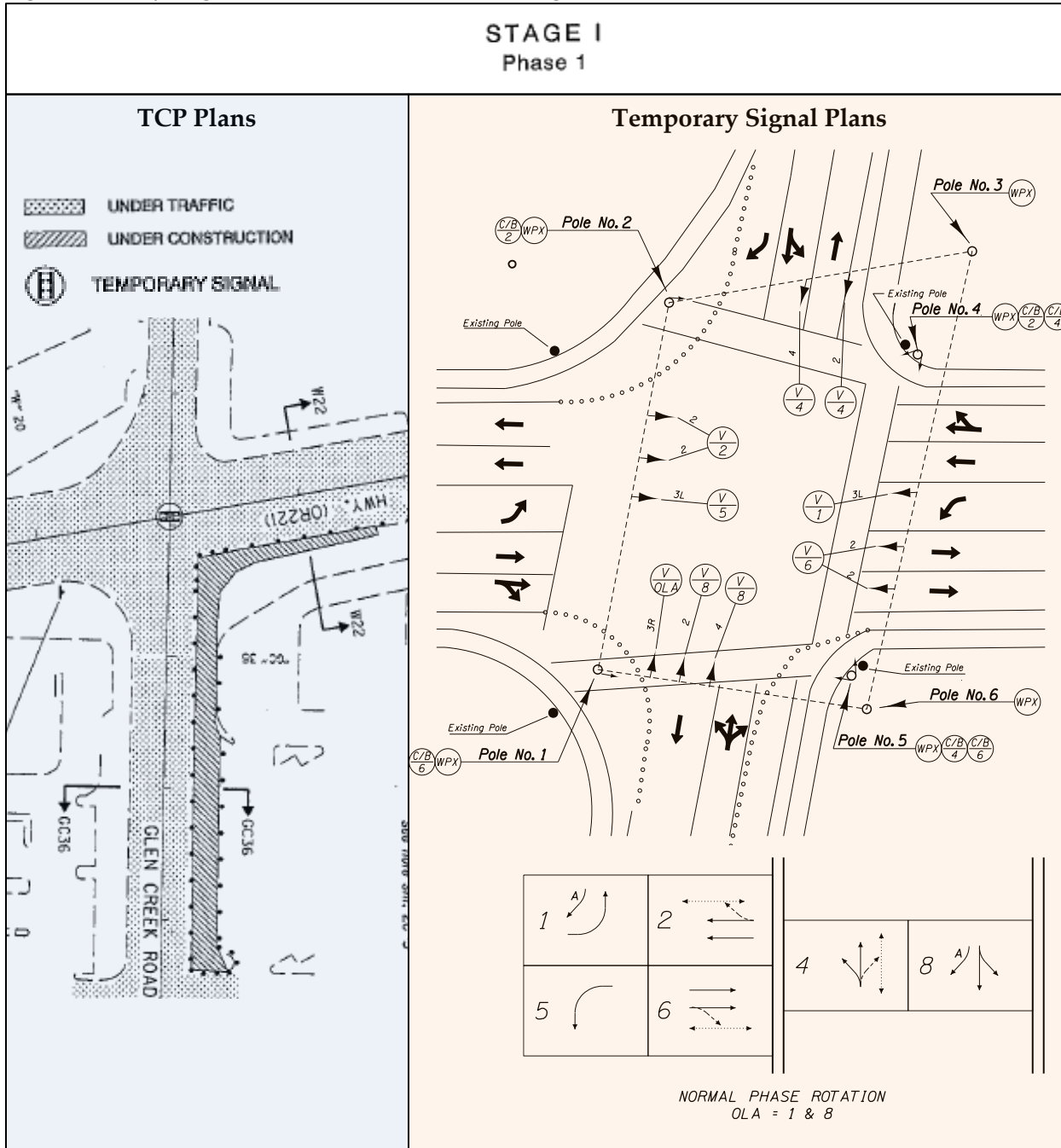
Figure 11-11 | Staged Construction Example – Stage I, Phase 1
