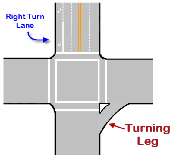
Figure 37: Turning Leg Diagram
