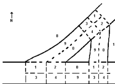
Intersection Type 3, with 2 turning legs
