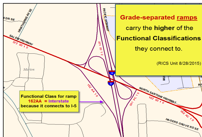
Figure 4: Grade Separated Ramps
