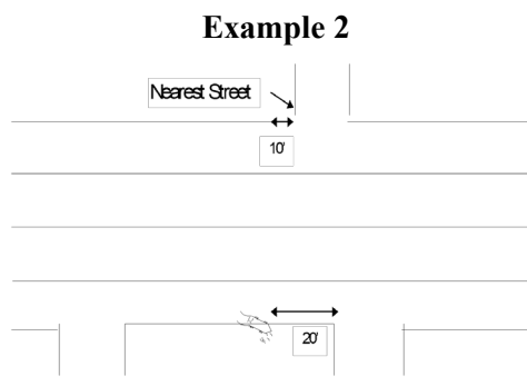
Figure 23: Undivided Highway
