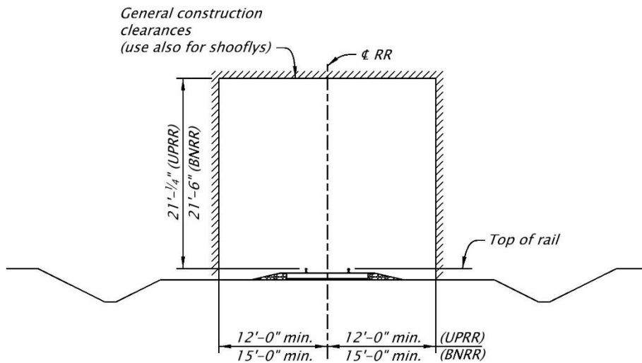
Figure 2.14.11.3-1 – Railroad Construction Clearances
