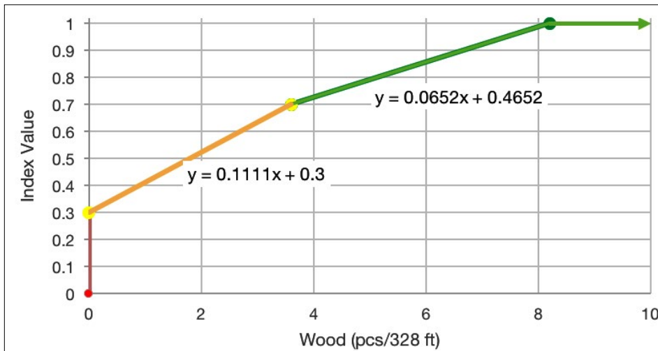
Figure 4.25 Wood Standard Performance Index - Western Mountain Ecoregion; > 50 ft width
