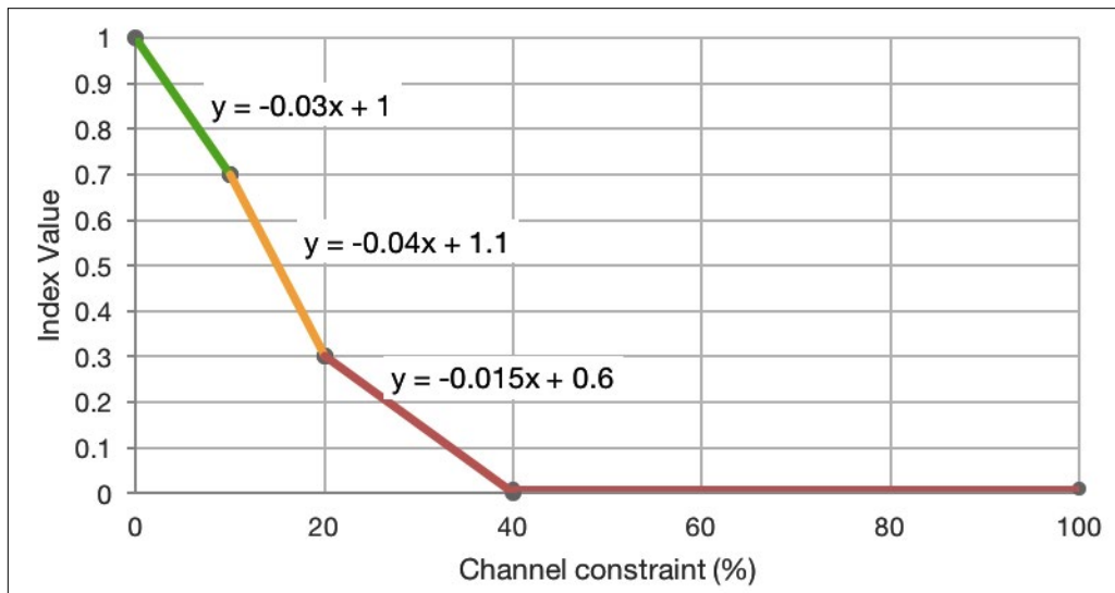
Figure 4.23 Lateral Migration Standard Performance Index
