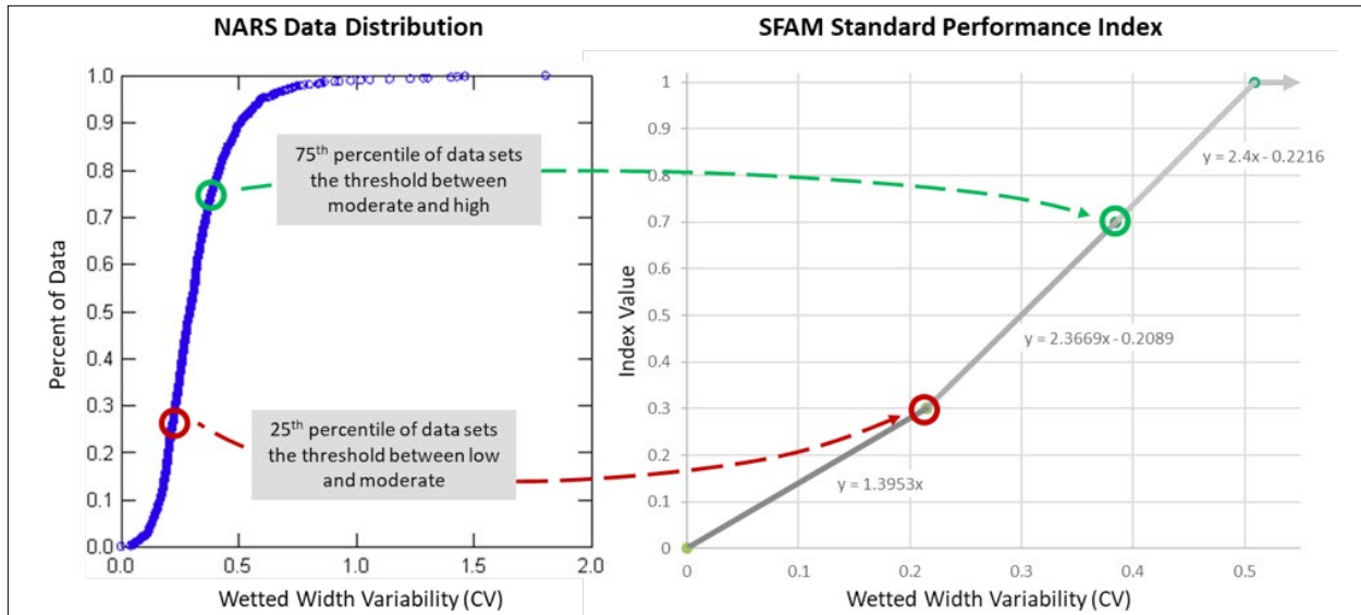
Figure 4.2 Raw Data Distributions from EPA NARS Surveys are Used to Set Performance Expectations
