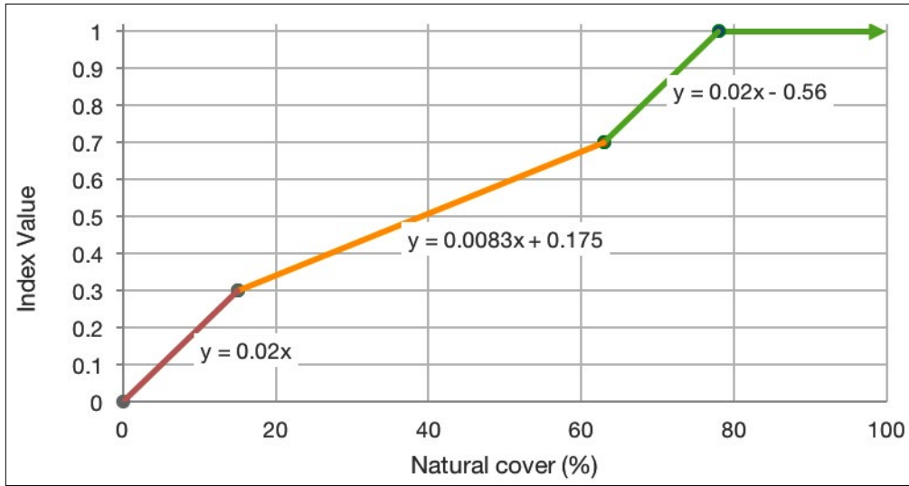
Figure 4.4 Natural Cover Standard Performance Index - Western Mountain Ecoregion; >50 ft width
