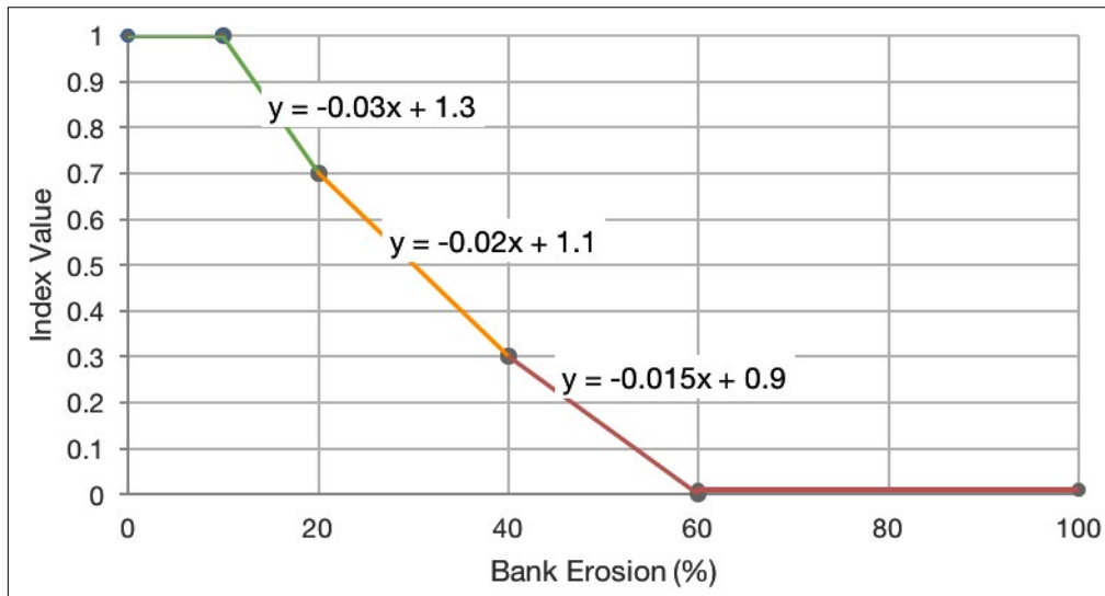
Figure 4.18 Bank Erosion Standard Performance Index
