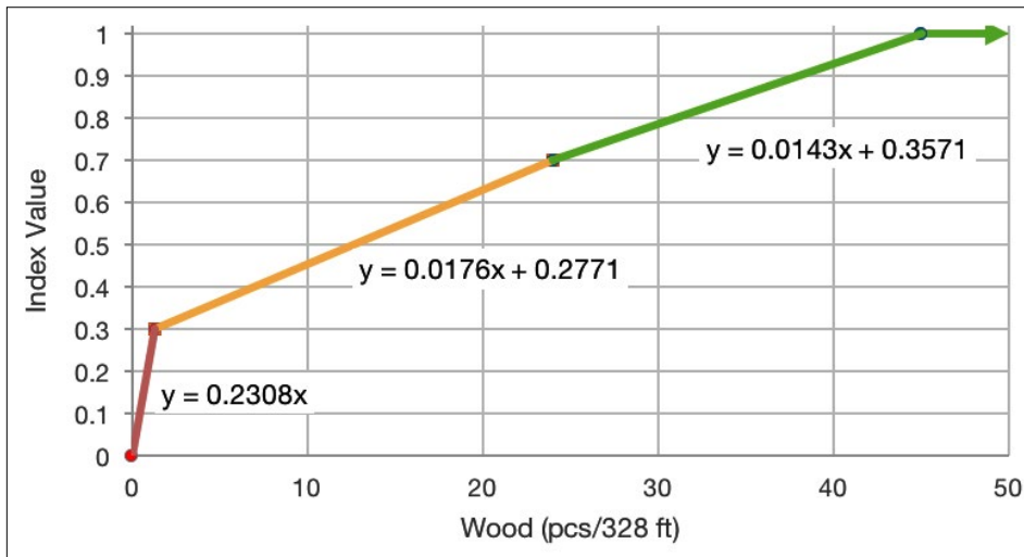
Figure 4.24 Wood Standard Performance Index - Western Mountain Ecoregion; ≤ 50 ft width
