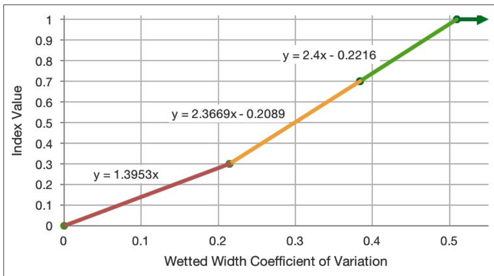
Figure 4.32 Wetted Width Standard Performance Index
