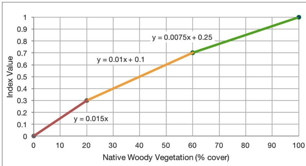
Figure 4.9 Woody Vegetation Standard Performance Index
