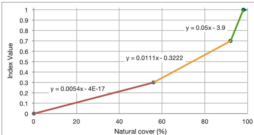
Figure 4.3 Natural Cover Standard Performance Index- Western Mountain Ecoregion; ≤50' width
