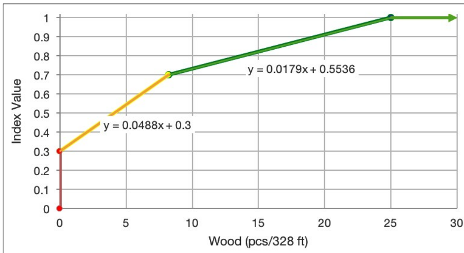
Figure 4.26 Wood Standard Performance Index - Xeric Ecoregion; ≤ 50 ft width
