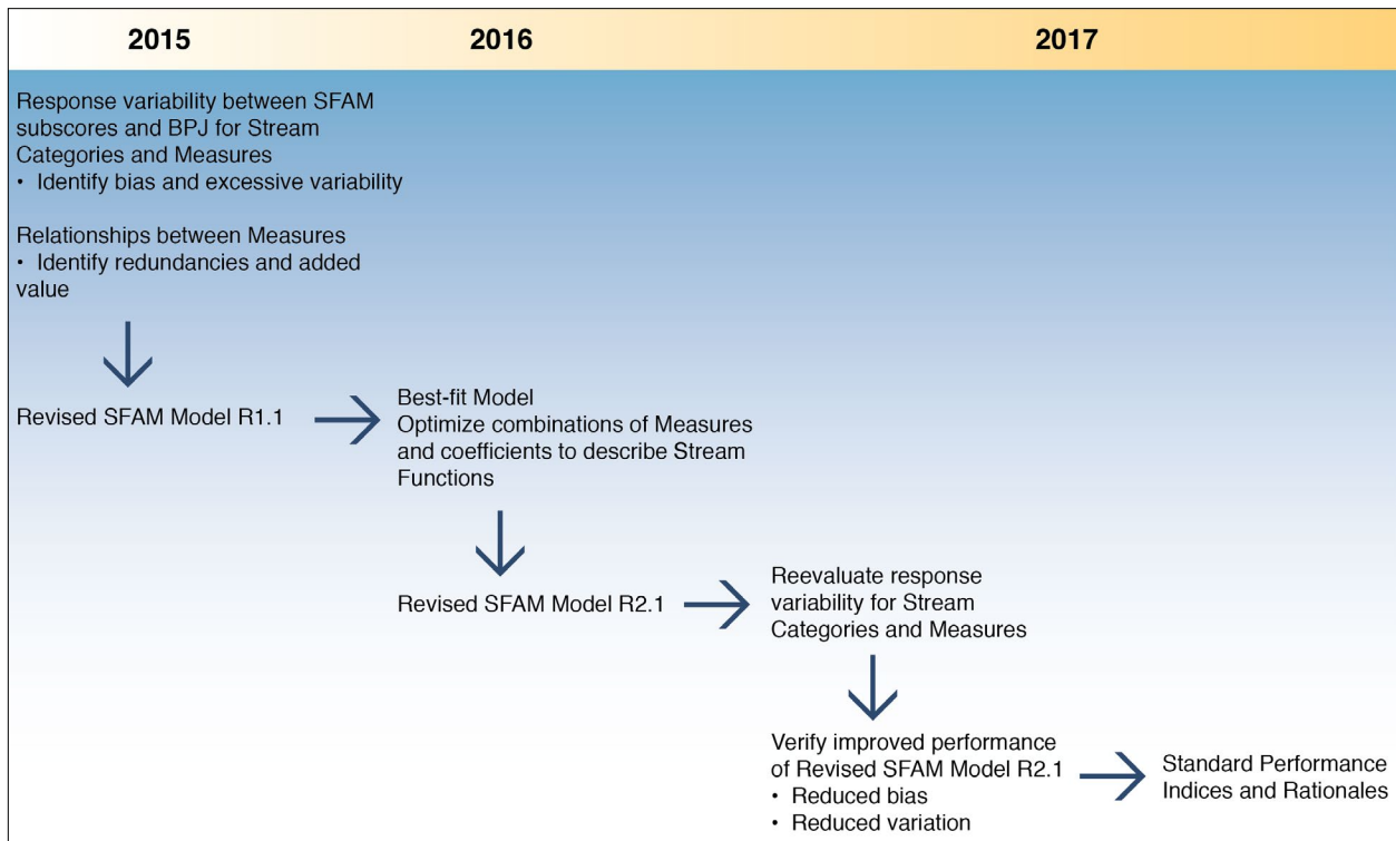
Figure 2.3 Procedure for Statistical Analysis
