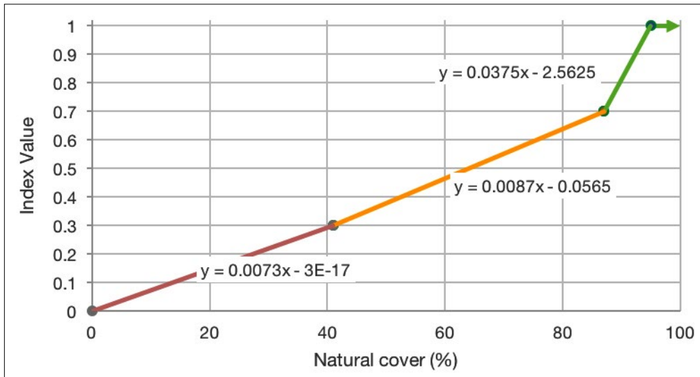
Figure 4.5 Natural Cover Standard Performance Index- Xeric Ecoregion; ≤50 ft width
