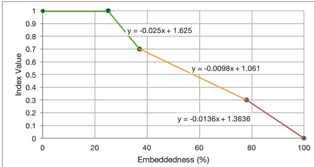
Figure 4.31 Embeddedness Standard Performance Index
