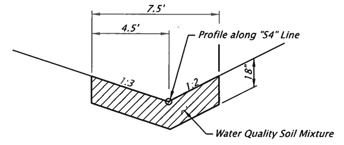
TYPICAL SECTION Scale: 3/16"=1'-0"
