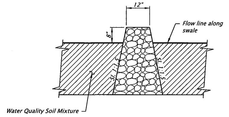
RIPRAP DETAIL No Scale
