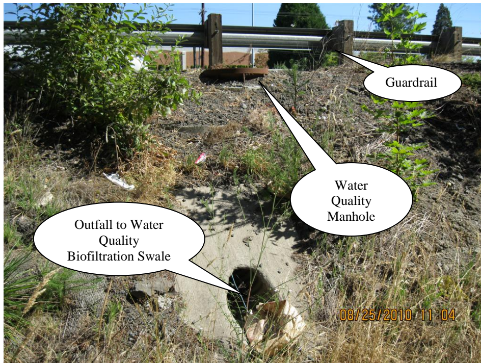
Photo 2: Water Quality Manhole and outfall pipe into Water Quality Biofiltration Swale (D00167).
