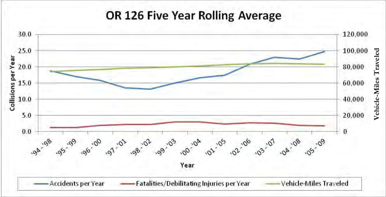
Figure 6.17. OR 126W Collisions Relative to Vehicle-Miles Traveled (Five Year Rolling Average)
