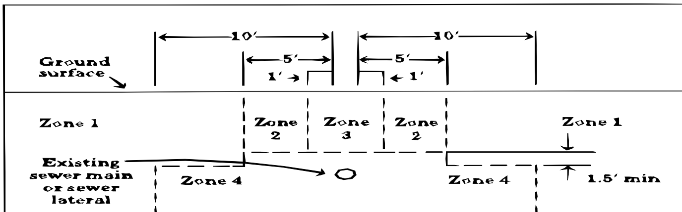
Figure 1: Water Line-Sewer Line Separation
