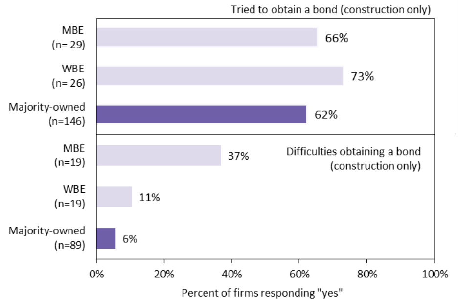
G-7. Responses to availability survey questions concerning bonding
